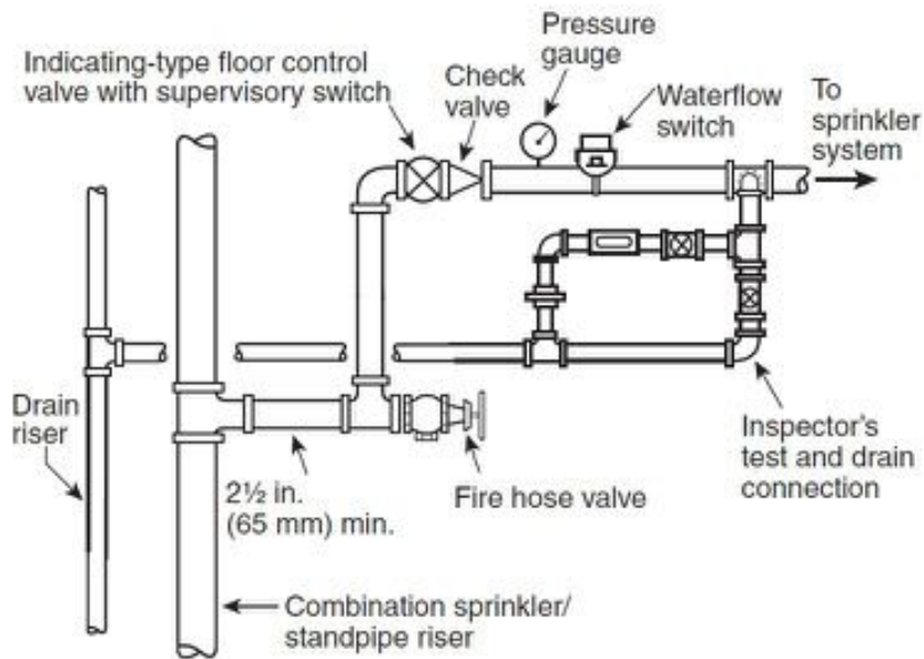
Combined Sprinkler/Standpipe System (NAPA 14, 2007 edition)
