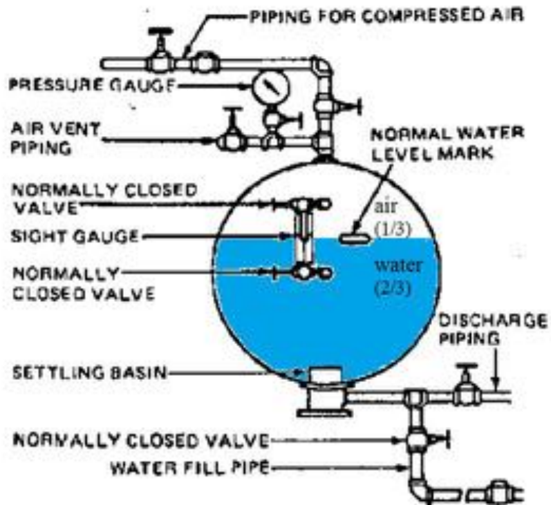
A Standard Pressure Tank
